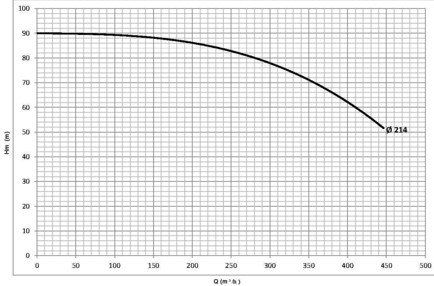
TKF 100-200 (3600RPM)
